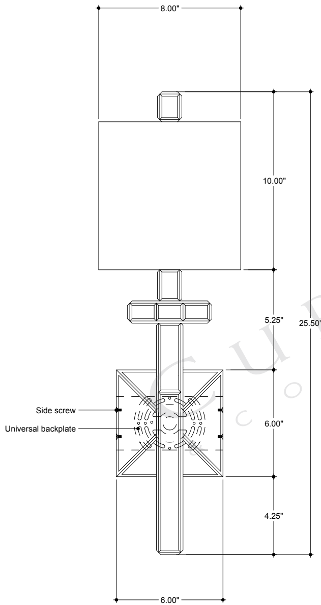
FRONT VIEW
